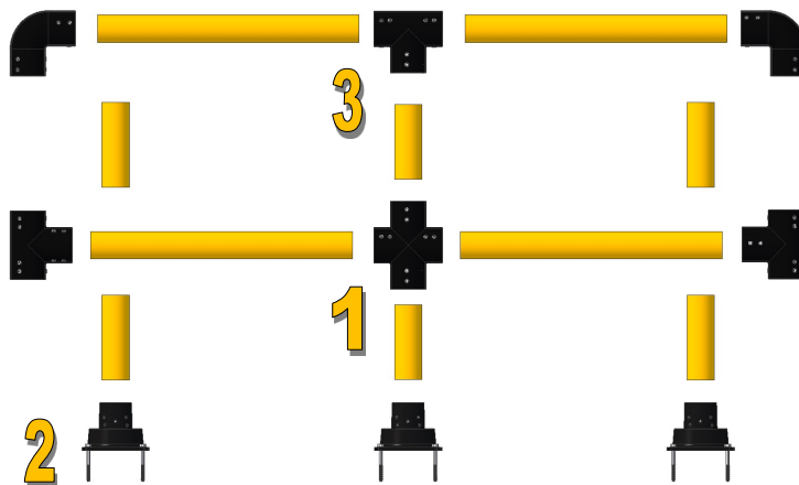
Double IronFlex Exploded View
